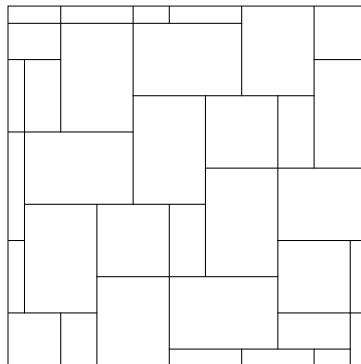
TLI_150_P_BCD_E1 Layout 5 (13% B - 25% C - 62% D)
